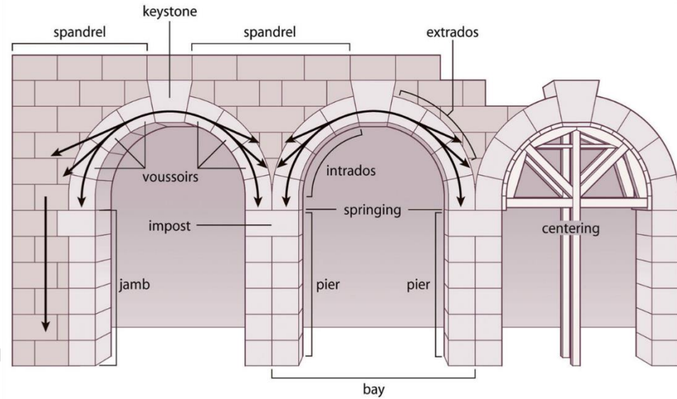
round arch
