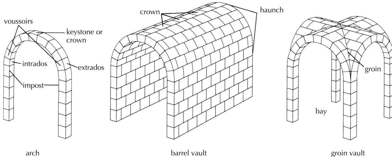
arch
